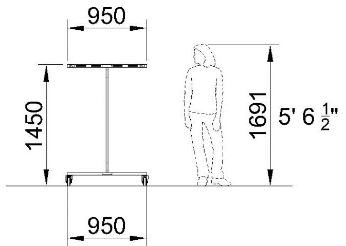
END VIEW
